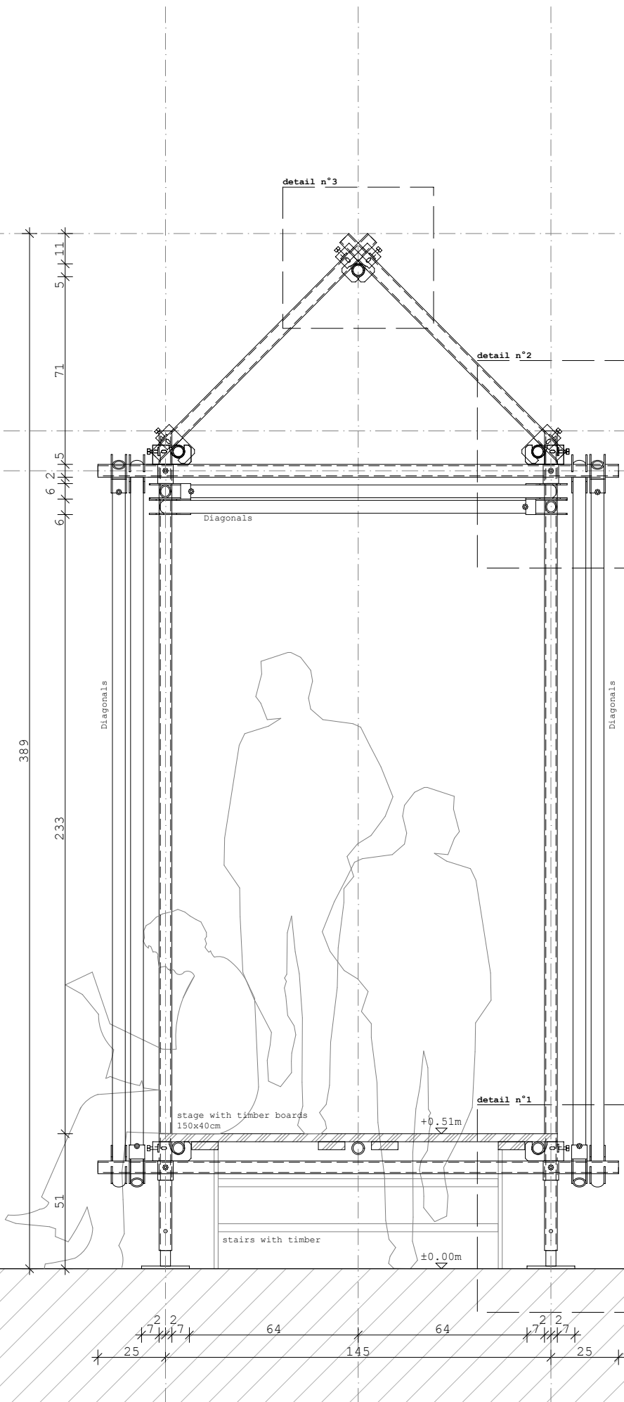
section 1:20
